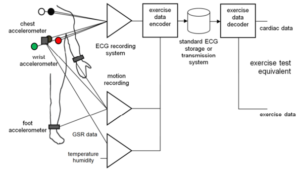
Fig. 1. Block diagram of home exercise monitoring system.
