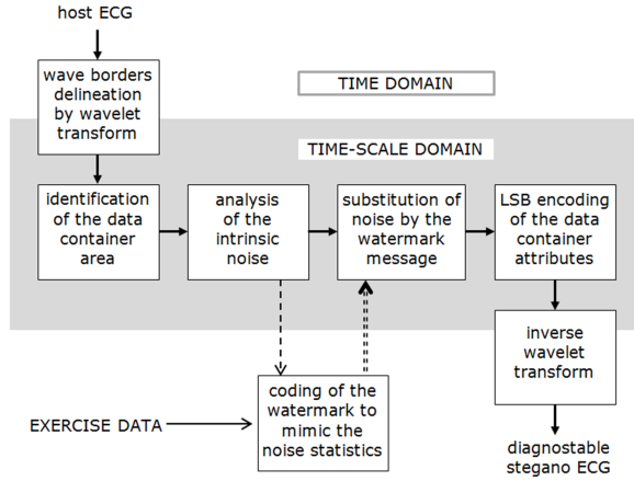
Fig. 2. Time scale ECG watermarking procedure.
