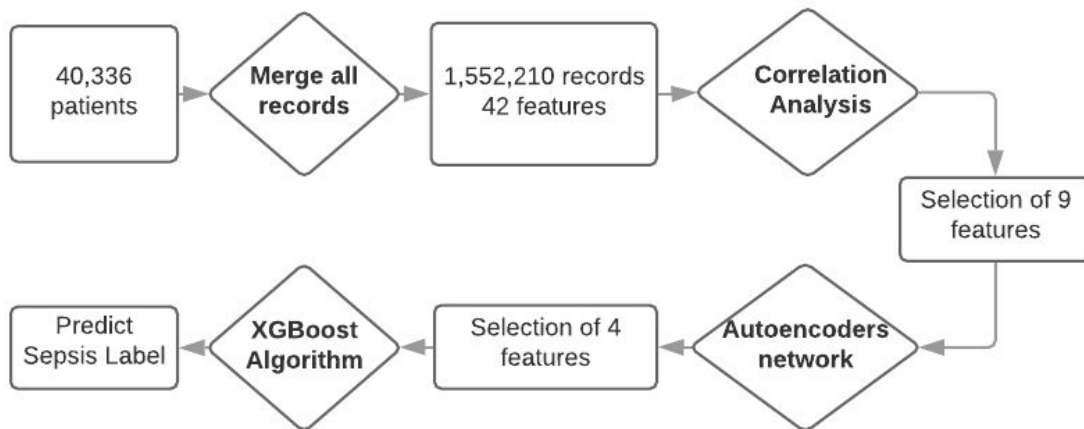
Fig 1. Framework for anomaly detection to predict sepsis from clinical data.
