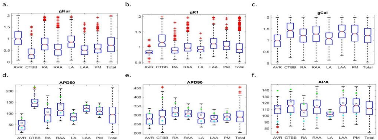
Figure 3 Boxplots showing regional variation of conductances and biomarkers compared with the values used in the standard Malekar model. a. shows the gKur conductance, b. shows the gK1 conductance, c. shows the gCal conductance, d. shows APD50, e. shows APD90 and f. shows APA
