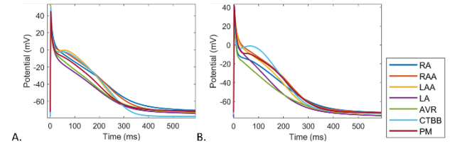
Figure 1 The mean action potential for regional populations. A. shows the mean action potential as calibrated by the experimental data, and B. shows the mean action potential of each regional population.
