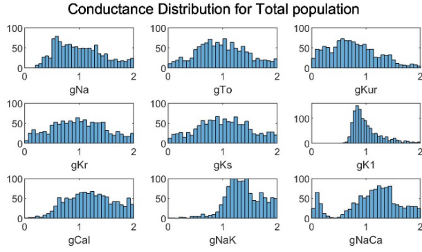
Figure 2 Histograms showing the distribution of the 9 varied conductances for the total population. From left to right the histograms show the distribution of gNa, gTo, gKur, gKr, gKs, gK1, gCal, gNaK, gNaCa respectively.
