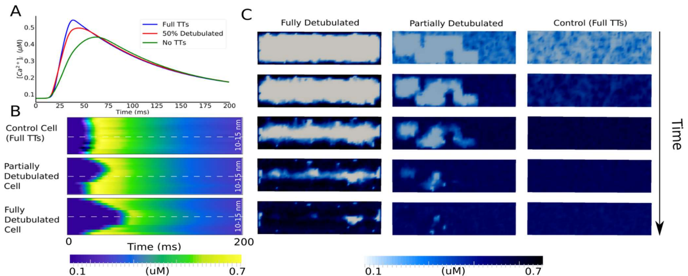
Figure 2 - Effects of detubulation on stimulated Ca^{2+} wave propagation. A) Intracellular Ca^{2+} transient for a fully, partially and none-detubulated cell in the stochastic model. B) Line scans along the X-axis of the cell over 200 ms. C) Intracellular Ca^{2+} snapshots along the Y-Z plane of fully, partially and none-detubulated versions of the stochastic rabbit atrial myocyte cell model.
