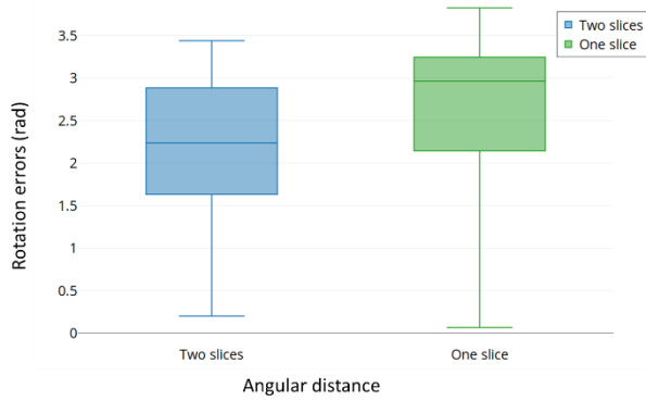
Figure 3 angular distance between the estimated rotations and the GT.
