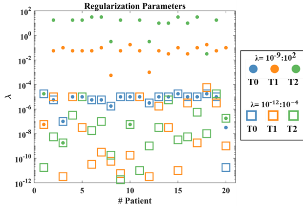
Figure 2. Results of the selected regularization parameters ( \lambda ) for a high range of \lambda (dots) and low range (squares) for zero, first and second order Tikhonov regularization (T0, T1 and T2, respectively).
