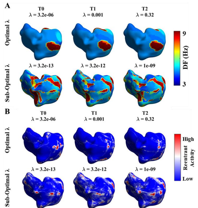
Figure 1. Dominant frequency (A) and singularity point maps (B) from an atrial fibrillation signal obtained by Tikhonov regularization of zero, first, and second-order (T0, T1, and T2). The first row of each panel represents the solution using an optimal regularization parameter ( \lambda ) and the second row a sub-optimal \lambda .
