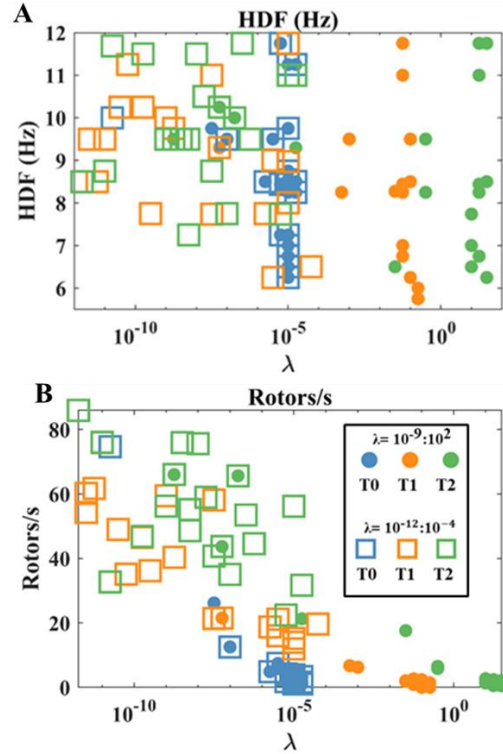
Figure 3. AF-related metrics obtained with the three TR orders versus the selected regularization parameters ( \lambda ) for a high range (dots) and low range (squares) of \lambda . A: Highest dominant frequency; B: rotors per second.
