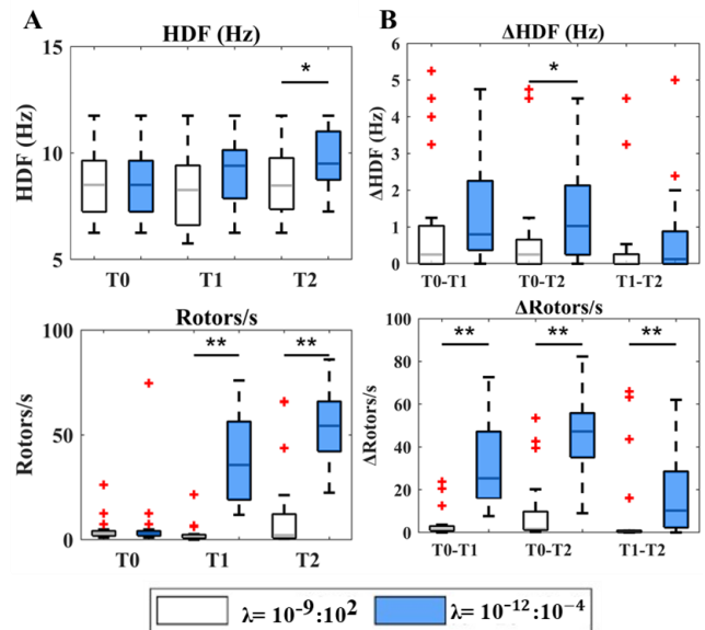
Figure 4. A. Comparison of ECGI metrics for each TR order for a high range of \lambda (white) and a low range of \lambda (blue). B. Comparison of the difference of ECGI derived metrics between TR orders and \lambda ranges.
