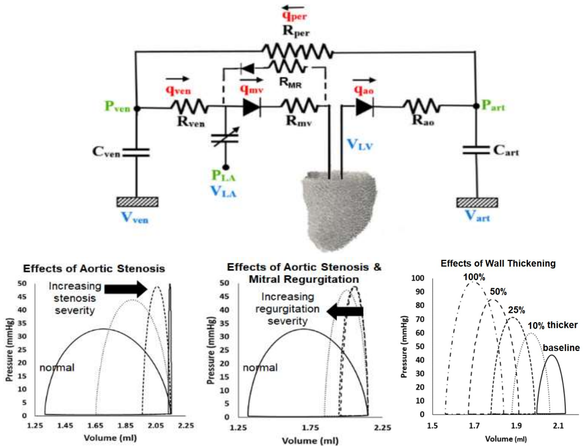
Figure 1: (Top) Schematic of FE and Windkessel model. (Bottom) Sample results of pressure-volume loops, during normal fetal heart conditions and during fetal aortic stenosis, mitral regurgitation, and LV wall hypertrophy.
