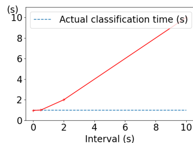
Figure 3: Mean classification time for varying interval in the threshold approach.
