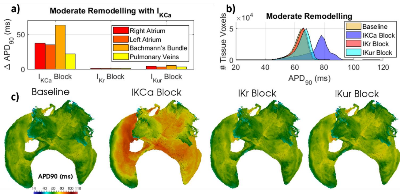
Figure 2. Effect of the 50% blockade of different ionic channels on APD 90 values for the atrial canine model [8] in the presence of I KCa (Eq. (1)) for moderate ionic remodelling. a) Increase in single-cell APD 90 for each cell type for each AAD (BCL: 500 ms). b) Histogram of APD 90 in atrial tissue in baseline conditions and after the administration of each AAD (BCL: 150 ms). c) APD 90 maps in baseline conditions and in the presence of each ionic channel blocker (BCL: 150 ms).
