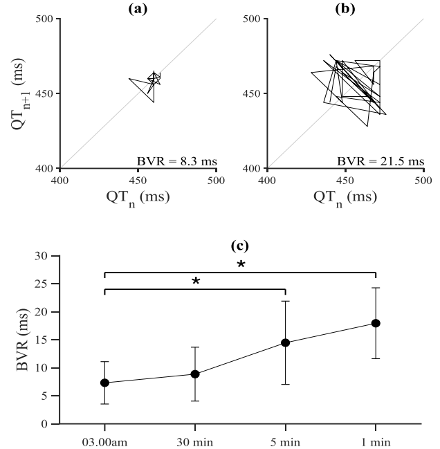
Figure 2: Poincaré plot of QT from a representative patient with IHD. Increased dispersion of the repolarization time, and thus the BVR values, from 03.00am (a) to 1 minute prior to nsVT (b) is clearly present. This increase is also found in the entire population for 1 minute and 5 minutes prior to nsVT (c). *p < 0.05 vs. 03.00am.
