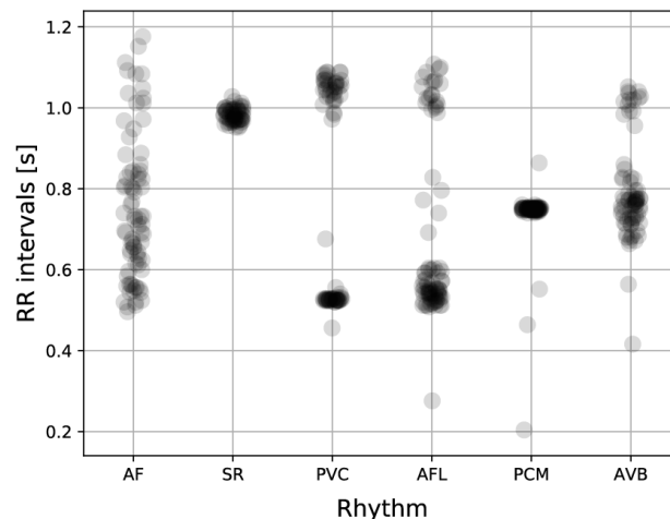
Figure 1. Examples of RR distributions in 60-second recordings of different rhythms. AF-Atrial Fibrillation, SR – sinus rhythm, PVC – premature ventricular contractions, AFL –atrial flutter, PCM – paced rhythm, AVB – 2 nd degree AV block
