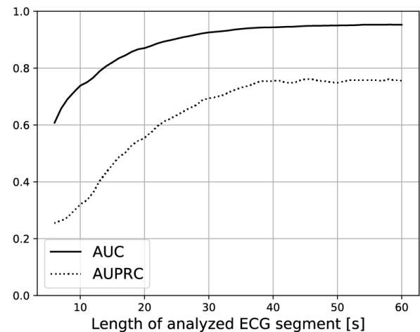
Figure 5. Method performance by the length of source ECG segment. AUC-area under the curve, AUPRC – area under the precision-recall curve. The performance was tested using 7,254 ECG segments from the private dataset.
