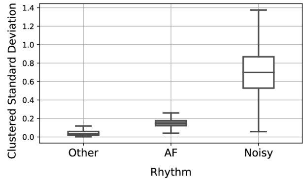
Figure 3. Clustered Standard Deviation could be used to detect noisy recordings if different clustering limits ( a=6 and b=0.04 ) are applied.
