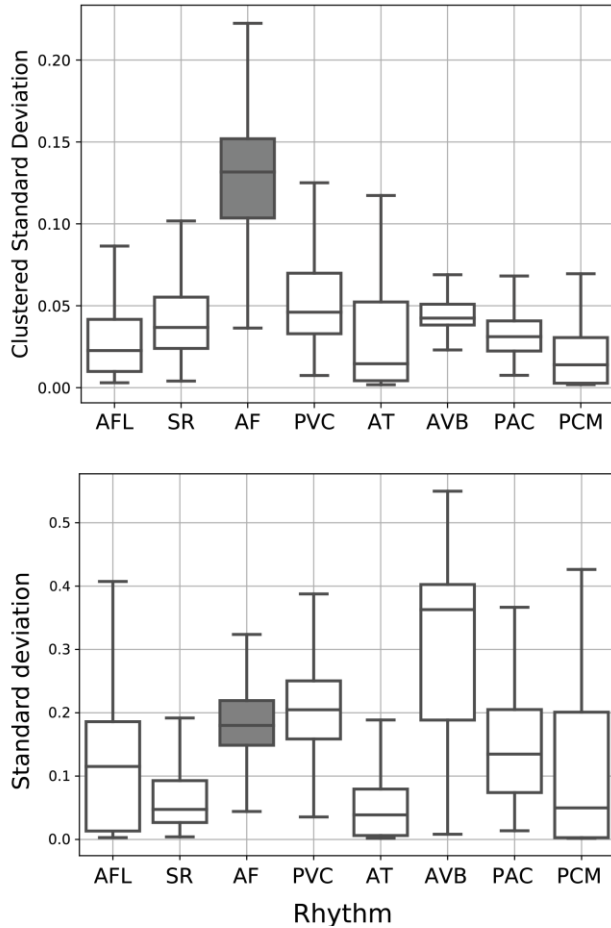
Figure 2. Comparison of the Clustered Standard Deviation (top) and the Standard Deviation (bottom) for different rhythms. Clustering limits were set to a=0.05 and b=0.06 . Private dataset (MDT, Brno, CZ) consisting of 7, 254 ECG segments was used. AFL-Atrial flutter, SR – sinus rhythm, AF-Atrial Fibrillation (gray), PVC – premature ventricular contractions, AT – sinus tachycardia, AVB – 2 nd degree AV block, PAC – premature atrial contractions, PCM – paced rhythm.
