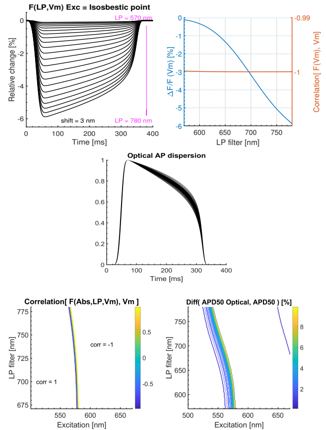
Figure 4. (Upper) Excitation at the isosbestic point for different LP filters (primary effect), E_{ms} = E_{ms}(LP + k*V_m) , integrated from each LP filter value to 900 nm. The fractional change is negative. 'Optical' V_m is fully correlated with 'Electrical' V_m for any LP. (Middle, lower) Primary and secondary effects, E_{ms}(Exc, LP, V_m) . Optical AP dispersion: normalized 'optical' APs for range of excitation wavelengths and LP filters. The correlation map shows a region for correlation < 0.99. Relative differences > 1 % between 'optical' APD50% and the 'Electrical' APD50%.
