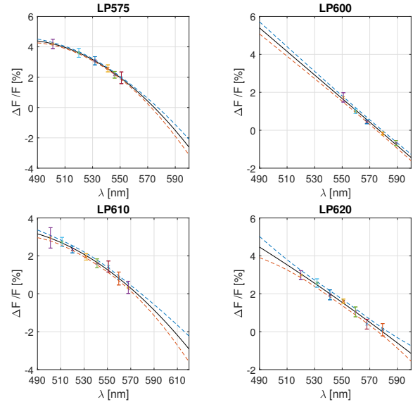
Figure 2. Relative changes of emitted fluorescence for four different LP filters of 575 nm, 600 nm, 610 nm and 620 nm for different excitation filters calculated as averages across all pixels. Quadratic polynomial fit curves are presented with 95% confidence interval range. Zero crossings correspond to the isosbestic point.
