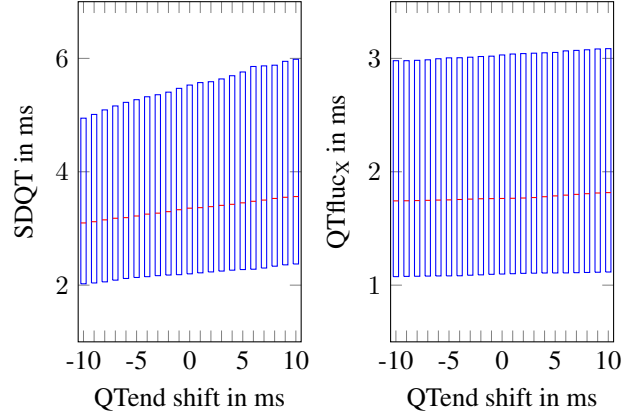
Figure 1. Standard deviation of QT intervals (SDQT) and QT fluctuation in time (QTfluc X ) for different delineations of the QT interval end (QTend) generated by shifting of the QTend boundary (QTend shift) in all datasets of the PTB diagnostic ECG database. Values are plotted as median and interquartile range.
