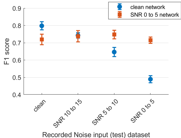
Figure 4. F1 scores for network trained using the 0 to 5 dB SNR Recorded Noise training data, and the network trained using the clean data, when classifying the Recorded Noise test datasets.
