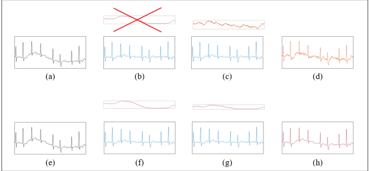
Figure 1. How the Recorded Noise (top) and Filtered Noise (bottom) datasets were generated. For the Recorded Noise dataset, (a) obtain raw data, (b) filter to obtain clean signal and noise, discard noise, (c) select segment of recorded noise and scale to specified SNR, (d) add recorded noise to the clean signal. For the Filtered Noise dataset, (e) obtain raw data, (f) filter to obtain clean signal and noise, (g) scale noise to specified SNR, (h) add scaled noise to the clean signal.
