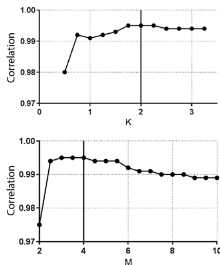
Figure 5. Optimization of coefficient K (top), affecting the influence of the S_{AD} . We also optimized coefficient M , affecting the removal of outlying QRS complexes (bottom). Performance was measured as a Pearson correlation between expert and automatically computed length of the longest pauses in the dataset.
