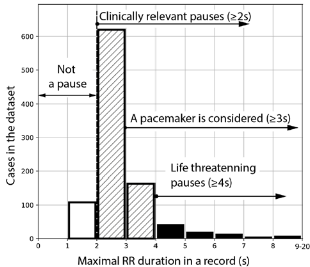
Figure 2. Distribution of maximal pauses in the dataset. Clinically relevant pauses (hatched and black) are equal or longer than 2s. Above three seconds, a pacemaker might be considered; life-threatening pauses (black) are longer than 4s.
