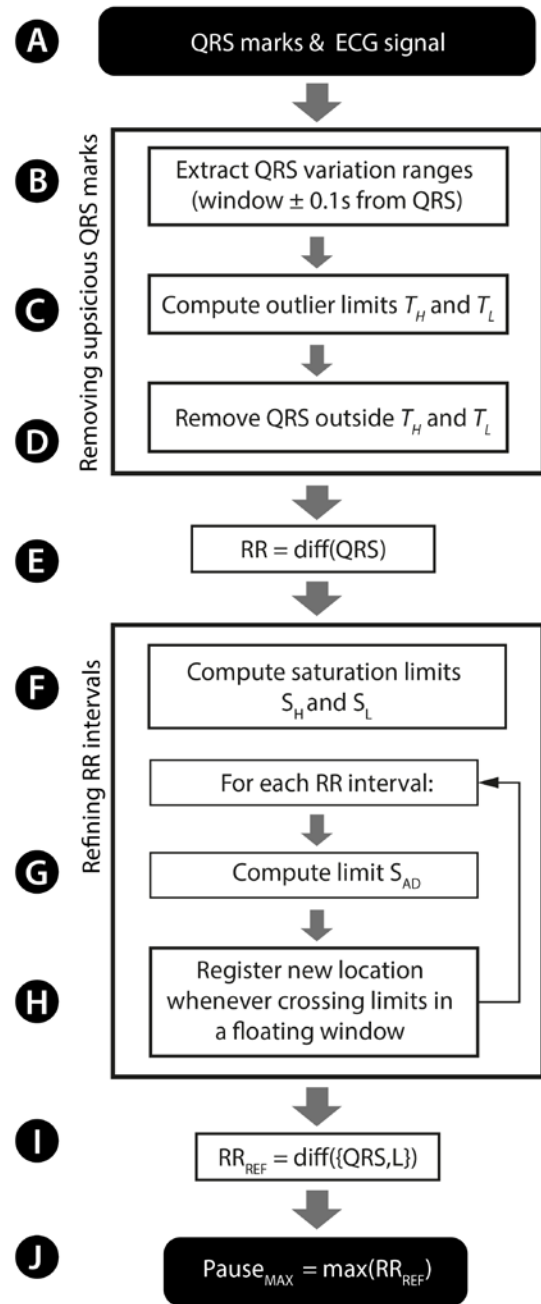
Figure 3. Method flowchart. QRS marks and ECG signal (A) are used to extract a list of variation ranges (B). Limits (C) are used to remove suspicious QRS marks from the list (D). Next, RR list (E) is acquired from QRS positions; saturation limits (F) are computed. For each RR interval, we compute the slope limit (G). We iterate through the RR interval and refine it whenever the signal properties exceed limits (H). Finally, we report maximal distance from the updated RR list (I) as a maximal pause (J).
