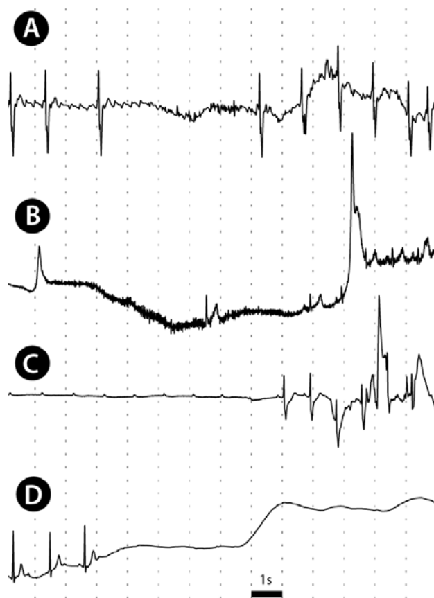
Figure 1. Examples of real pauses in Holter ECG signals. A 5s pause during atrial flutter (A), the end of 19s pause (sinus arrest) followed by another 3s pause (B), end of 12s pause during 2nd degree AV block (C). D shows a start of 13s long SA pause.
