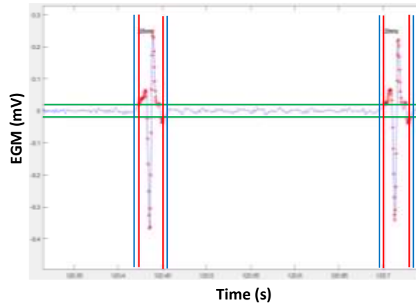
Figure 4. Example of EGM segmentation. The signal has been acquired with the the Advisor™ FL Circular mapping catheter.
