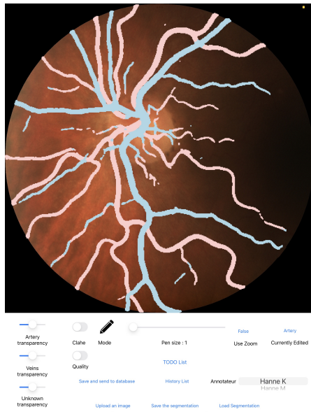
Figure 3. User interface of Lirot.ai-app including a pre-segmentation generated by our baseline model.
