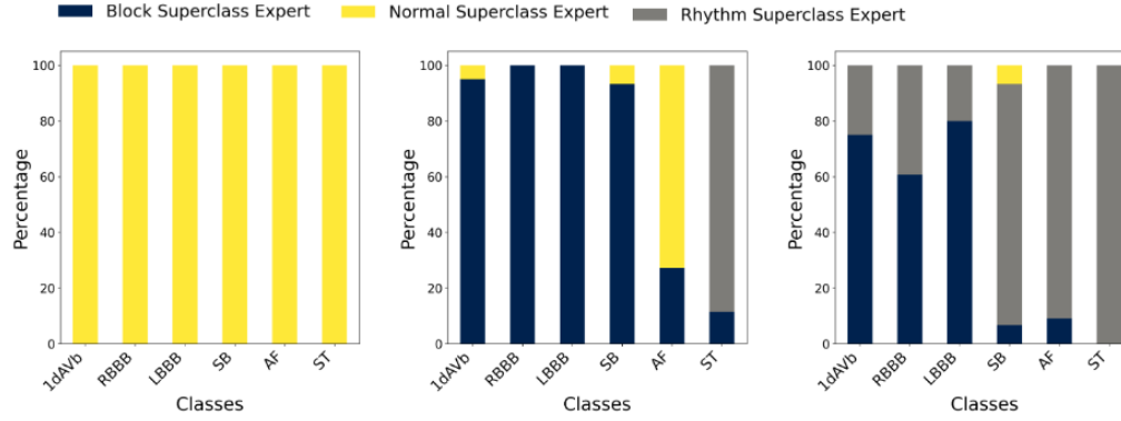
Figure 2. Percentage of each class classified by each expert by the gate from left to right: (a) MoE, (b) MoE Gate, (c) MoE GateC.
