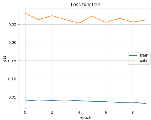
Figure 4. Loss function at each epoch.
