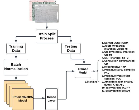
Figure 3. Proposed workflow for classification of ECG images.
