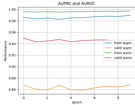
Figure 5. Plot showing the area under Precision Recall and Receiver Operating Characteristic curve.
